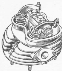
A feature of the cast-iron cylinder head is that the rocker pivot pins form part of a single forging that is bolted to the main casting
