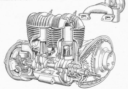
Of 244 c.c. (50 x 62 mm), the Excelsior Talisman twin cylinder two-stroke has two equally tapered cylinder barrels and cylinder heads. Each piston carries about 100 cc of oil. Crank throws are set at 150 degrees to provide the torque of a four-cylinder four-stroke. Five bearings support the crankshaft.
