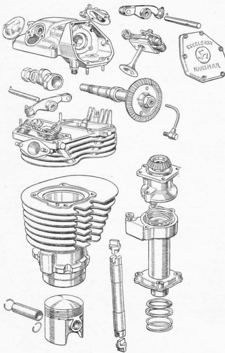
The cylinder finning of the "Manxman" engine is unusually deep and widely pitched. There is a positioning dowel for cylinder to head and cylinder to crankcase, the latter forming an oil lead to the rear of the cylinder. The drawing also shows the "overlapping" hairpin valve springs and details of the overhead camshaft gear
