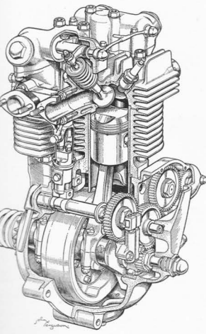
Called the Thunderbird, the 650 c.c. Triumph engine is a development of the Speed Twin and is notable for its high torque at comparatively low r.p.m. Bore and stroke are 71 x 82 as against 62 x 80 for the Grand Prix, Speed Twin and Tiger 100. Specially strong connecting rods, in R.R.56 light alloy, are fitted
