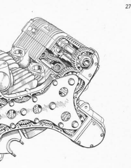
An outrigger plate supports the spindles of the camshaft drive pinions. The gear meshing with the crankshaft half-time pinion also drives the duplex gear oil pump and magneto.
