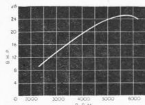
Power curve of the 495 c.c. A7 twin
