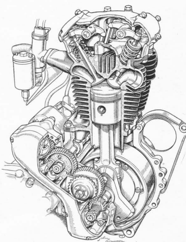
Big brother of the 500 c.c. A7, the 650 c.c. (70 x 54 mm) B.S.A. Golden Flash engine has larger diameter timing- and drive-side shafts and, also in keeping with the greater engine capacity, even more effectively cooled cylinder heads. Connecting rods are of light alloy. Unusual nowadays, the pistons have concave crowns. The tappets are of barrel type with chilled rubbing surfaces.
