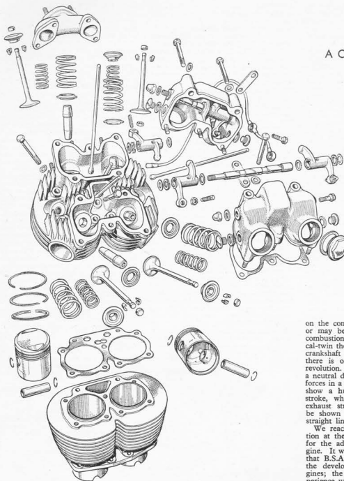
Two separate valve-spring wells, with an air space between them, are formed in the cylinder-head casting. The head is retained by nine bolts, one of which is in the middle to prevent distortion and give a good joint seal. Light-alloy rocker boxes are bolted independently to the head. Rockers operate direct on the steel spindles.
