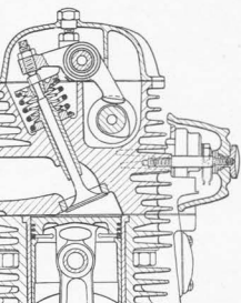
Detail construction of the shaft-drive and plunger-type rear suspension
