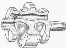
The one-piece alloy-iron crankshaft. Steel discs close the ends of the coring through the crankpin to suit the one of the discs incorporates a spring-loaded oil-release ball valve
