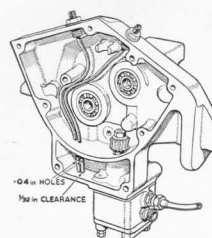
A double-acting oil pump is driven by worm gear.
