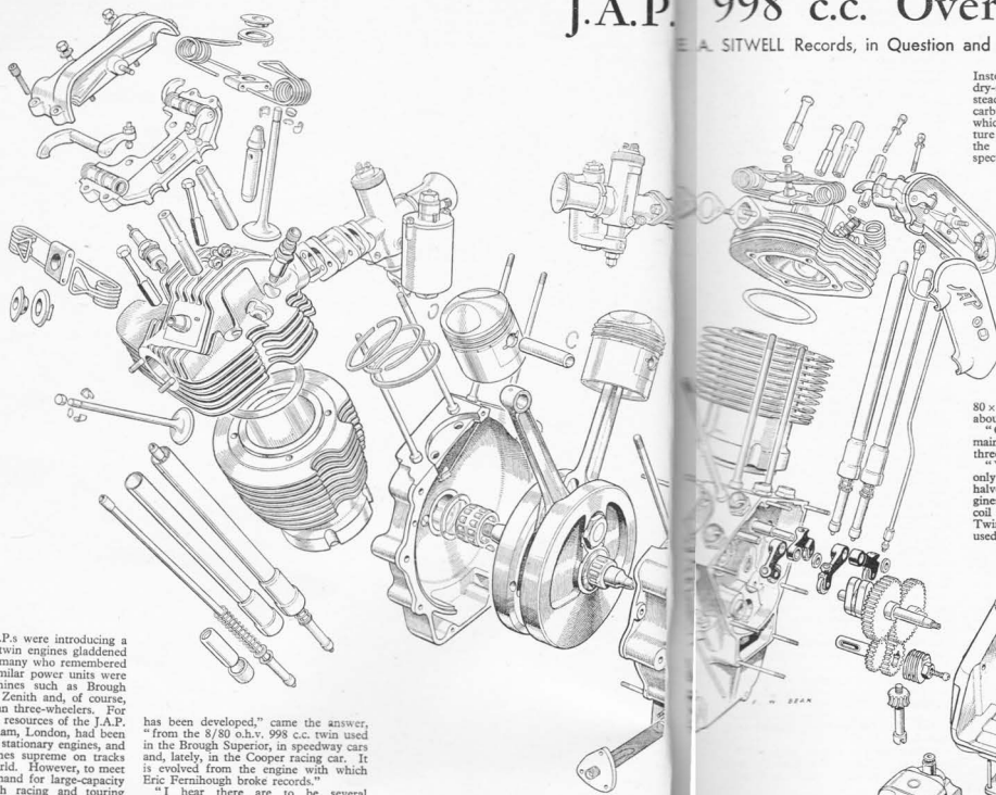
The new J.A.P. 998 c.c. vee-twin has light-alloy cylinder heads and cylinder jackets, the latter with cast-iron liners. Valve springs are of the duplex hairpin type
