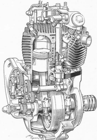
Called the Thunderbird, the 650 c.c. Triumph engine is a development of the Speed Twin and is notable for its high torque at comparatively low r.p.m. Bore and stroke are 71 x 82 as against 62 x 80 for the Grand Prix, Speed Twin and Tiger 100. Specially strong connecting rods, in R.R.56 light alloy, are fitted
