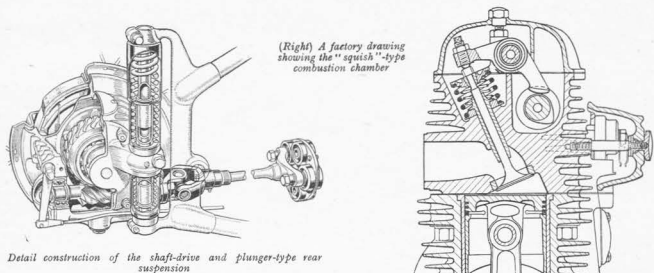
Detail construction of the shaft-drive and plunger-type rear suspension
