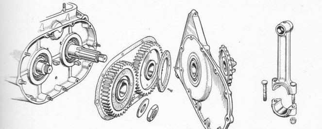
The two crankshafts are geared together, and the steel gear wheels have pressed-in and riveted fibre discs to prevent rind. The gear cover also forms the back plate of the primary chain case
