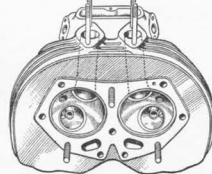
Separate induction ports are employed. Combustion chambers are unusually shallow.
