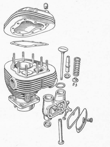
A detachable aluminium-alloy cylinder head is employed. The manner in which the detachable valve-spring housings are insulated from the cylinder and the division between exhaust- and inlet-port finning
