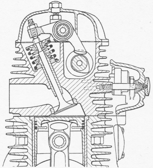
(Right) A factory drawing showing the "squish"-type combustion chamber
