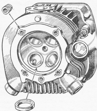
The light-alloy head is of the "semi-radial" type, the inlet side being flat and the exhaust side a portion of a sphere
