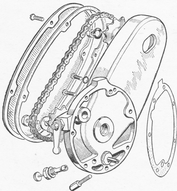
Details of the timing gear and oil-pump assemblies. The cams are integral with the shaft, which also incorporates a decompressor cam. Chain drive is employed for the magneto
