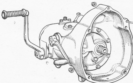
Engine and gear box are in unit. There is a single 7-in-diameter clutch friction plate. The kickstarter operates through a skew gear
