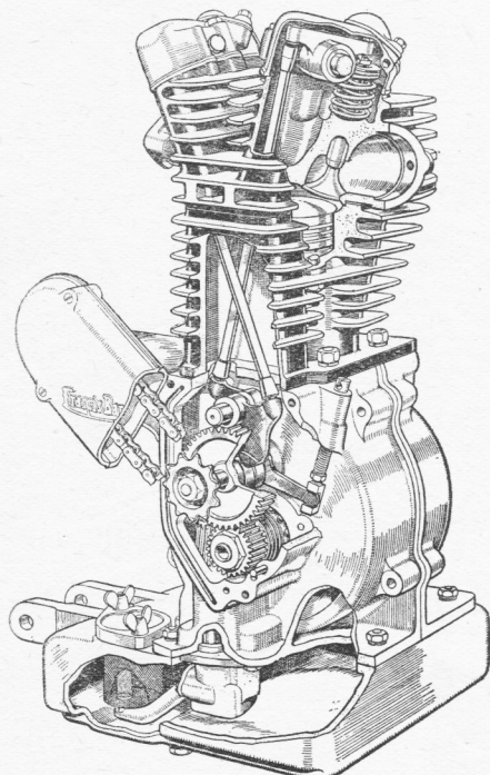
An interesting contrast with the C11 B.S.A.—the 247 c.c. (68 × 68 mm) Francis-Barnett "Stag," introduced for 1935
