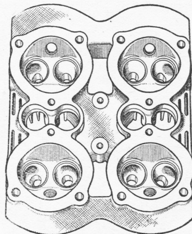
Each cylinder head is of pent-roof formation and houses two vertical valves
