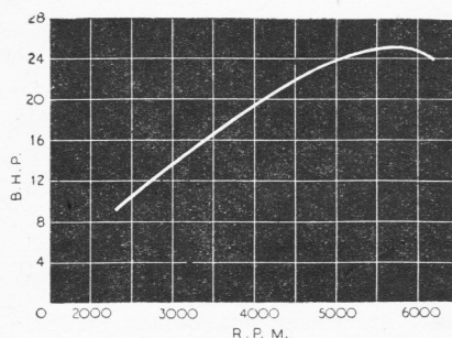
Power curve of the 495 c.c. A7 twin
