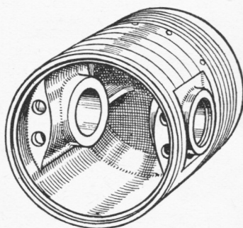
This view of the alloy piston shows how the casting is relieved at the bosses. Two narrow pressure rings and a scraper ring are employed
