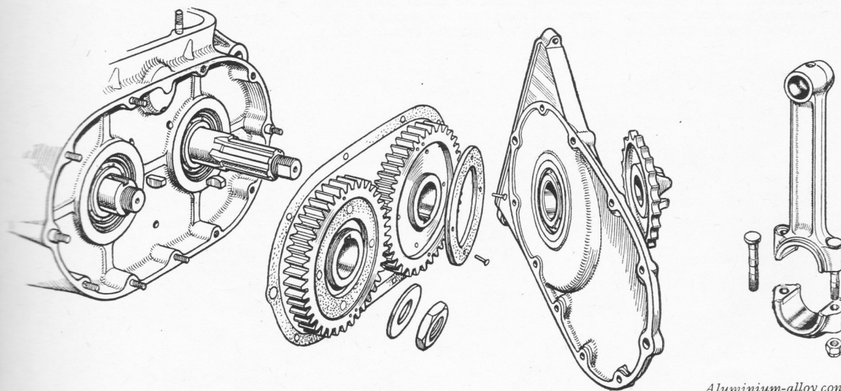
The two crankshafts are geared together, and the steel gear wheels have pressed-in and rimmed fibre discs to prevent ring. The gear cover also forms the back plate of the primary chain case
