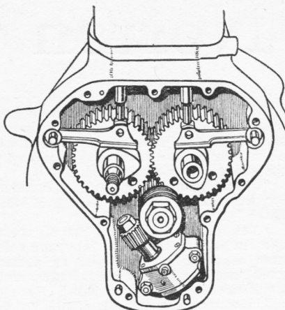
The drive for the timing gear is from the crankshaft to the exhaust camshaft and thence to the inlet camshaft. A worm drive is used for the oil pump
