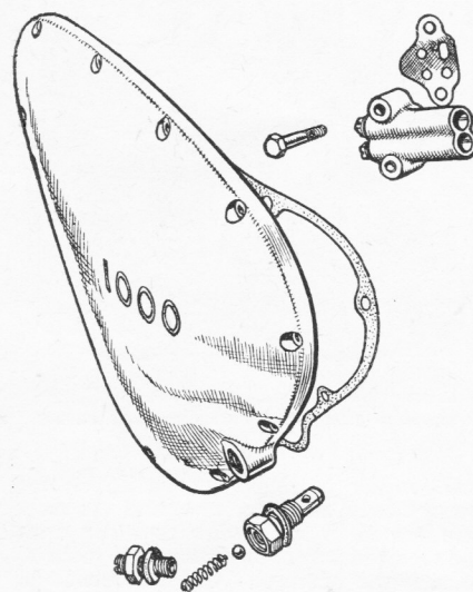
Both camshaft and Magdyno are driven by a single Weller-tensioned chain. The drawing also shows the oil pump, the oil filter and the relief valve in the timing-case cover
