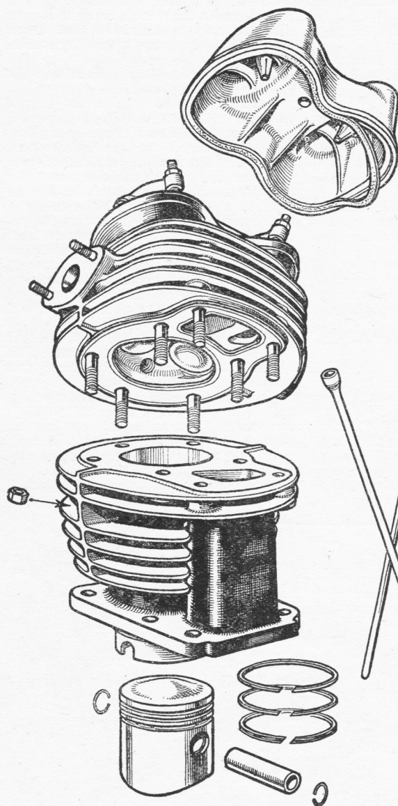
(Left) A copper-asbestos washer is used between the cylinder and head; the latter has a seven-stud fixing. The cone-shaped projections in the valve cover are breathers
