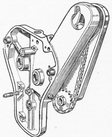
A spring-loaded gland in the timing-gear cover plate is a feature of the lubrication system. By means of this gland, oil is forced along the crankshaft into the big-end bearing
