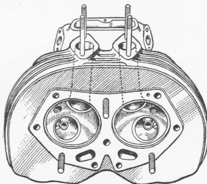
Separate induction ports are employed. Combustion chambers are unusually shallow
