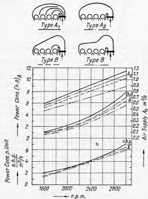
FIG. 303. Suitable shape of air duct.
