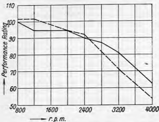
FIG. 167. Effect of varying valve size upon the desired octane number.
