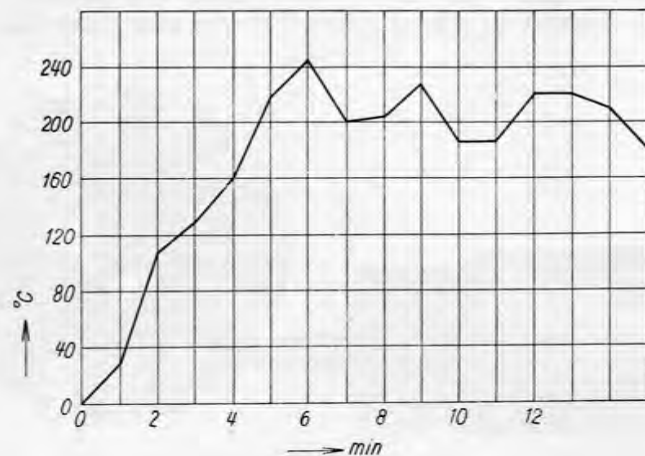
FIG. 112. Cylinder head temperatures after starting the Tatrapian engine with the Scintilla electro-magnetic coupling.
