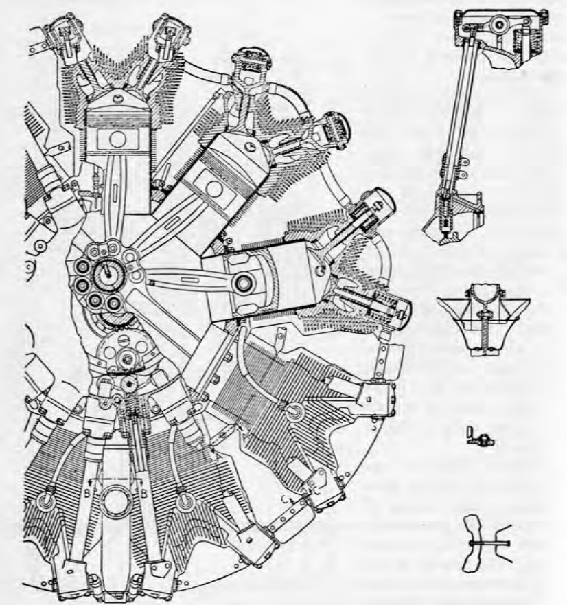
FIG. 203. Transverse section of a radial aircraft engine (Lycoming). Note the valve gear.
