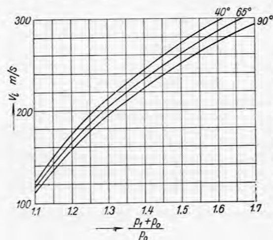
FIG. 342. Chart for the determination of the v_i/S ratio from the pressure ratio (p_1 + p_0)/p_0 for different temperatures of the scavenging air.
