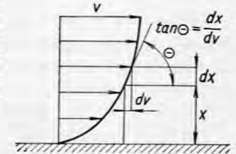
FIG. 29. Velocity profile of the boundary layer.
