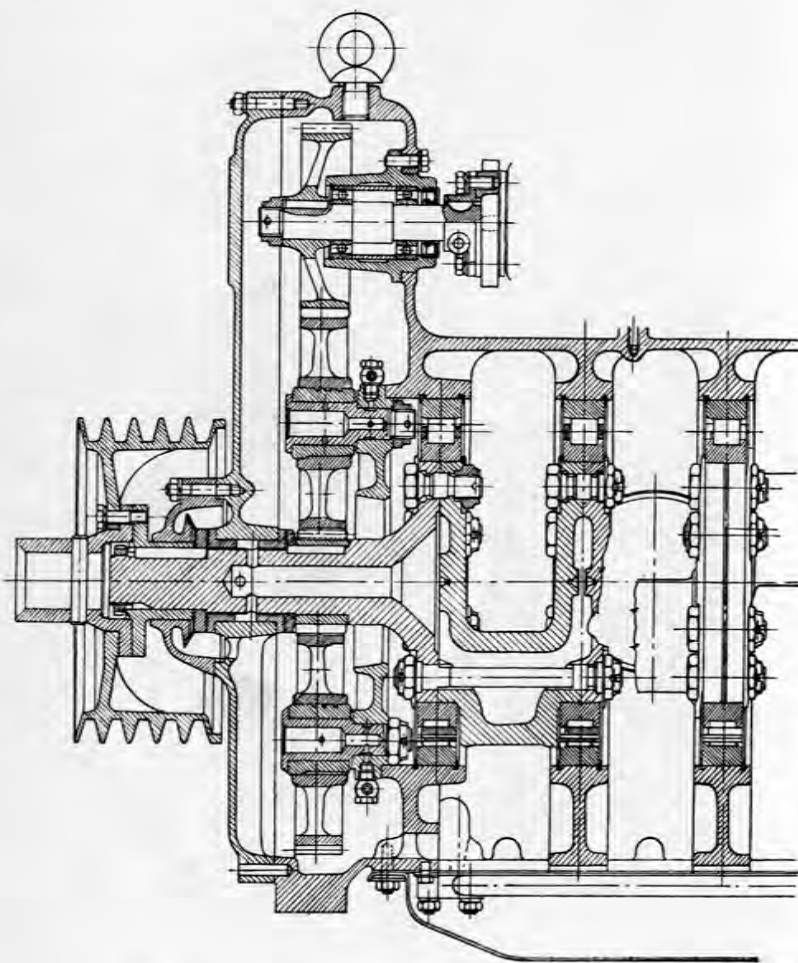
FIG. 411. Longitudinal section of the Tatra 116 engine.
