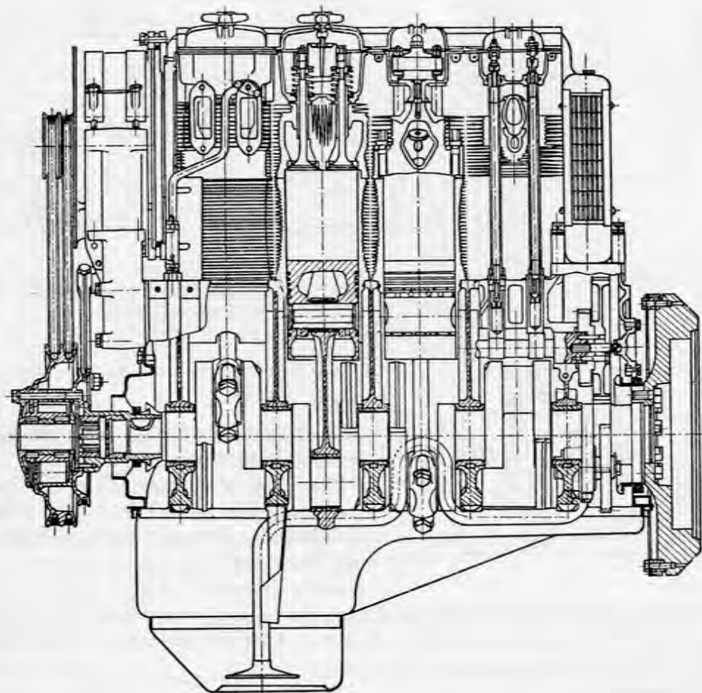
FIG. 216. Longitudinal section of the Deutz F-4-L-514 engine.
