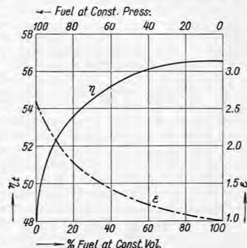
FIG. 190. Comparison of thermal efficiency according to fuel combustion at constant volume or constant pressure. The full curve represents efficiency, the dashed the expansion ratio \epsilon_e during combustion.
