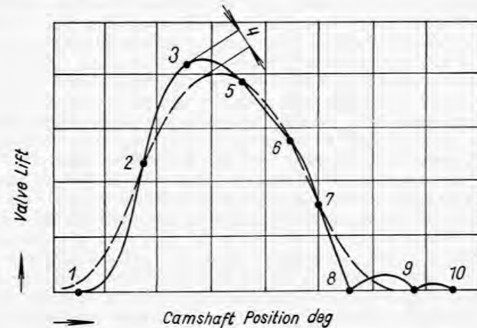
FIG. 288. Theoretical (dash line) and real (full line) course of the valve lift showing the effect of valve gear resilience.
