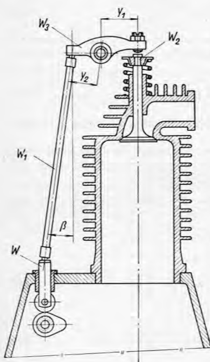
FIG. 281. Illustration of valve gear.
