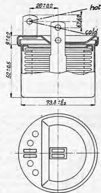
FIG. 129. Alcohol thermostat.
