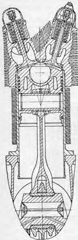
FIG. 397. Section of a cylinder of the MAN compression-ignition engine.
