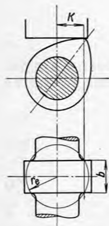
FIG. 268. Minimum diameter of the harmonic cam follower.
