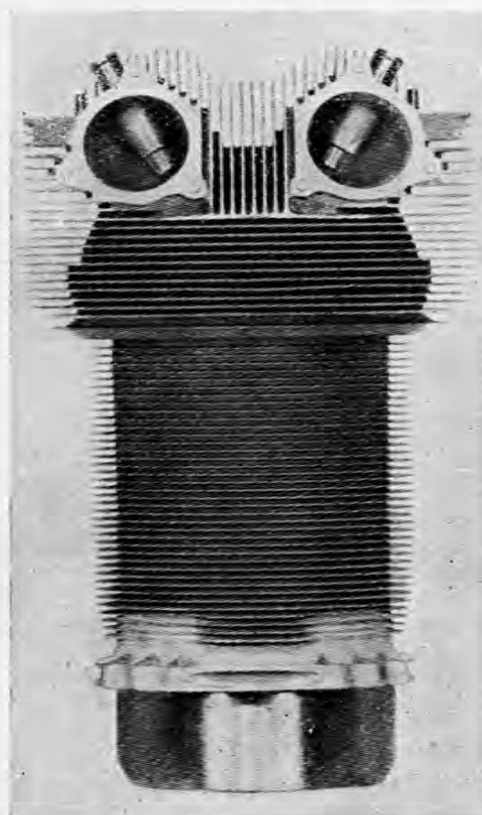
FIG. 209. The four-valve cylinder of the Bristol aircraft engine.
