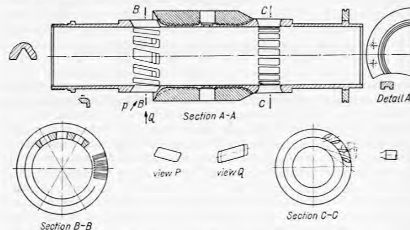
FIG. 360. The final one-piece design of the Orion cylinder.
