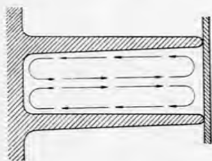
FIG. 72. Double vortex in the fin interstice due to friction between air and fin surface.
