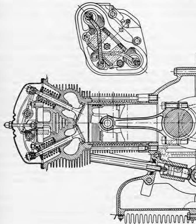
FIG. 103. Cylinder of the air-cooled Tatra engine. The inclined plane of the valves improves the passage of cooling air.
