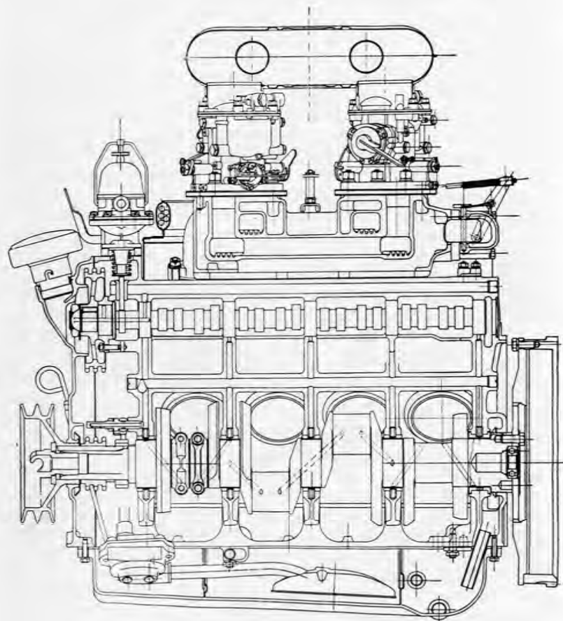
FIG. 339. Longitudinal section of the Tatra 603 F engine.
