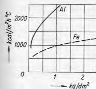
FIG. 82. Relation between heat transfer coefficient and unit weight of fins at a pressure head of 100 mm w.g.
