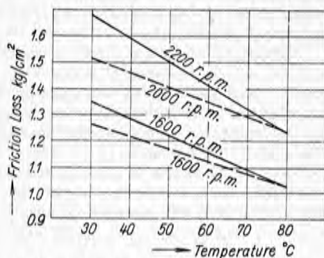
FIG. 104. Influence of cylinder (cooling water) temperature upon the average loss of pressure in a twelve-cylinder engine with 114.3 mm bore, 152.4 mm stroke and a compression ratio of 5.3 : 1 (full line). The dash line represents friction loss in an eight-cylinder engine, bore 140 mm, stroke 150 mm and compression ratio 5.4 : 1.
