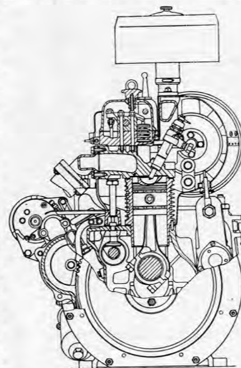
FIG. 401. Transverse section of the Petter engine.
