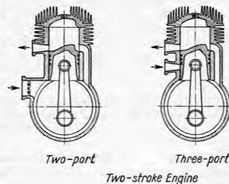
FIG. 331. A two-port and three-port two-stroke engine.
