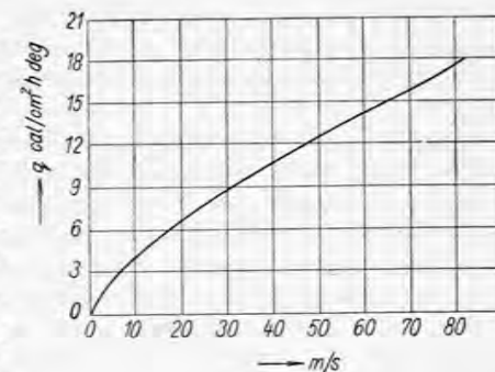
FIG. 34. Surface coefficient of heat transfer measured on an even surface in relation to air velocity.
