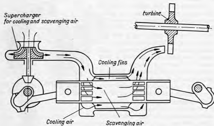
FIG. 358. Arrangement of air supply in a two-stroke aircraft engine.
