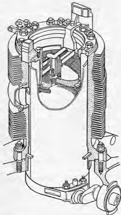
FIG. 296. Final design of the cylinder of the Bristol sleeve valve engine.
