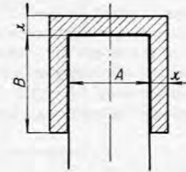
FIG. 90. Surface area around the cylinder for heat transfer to the cooling medium.
