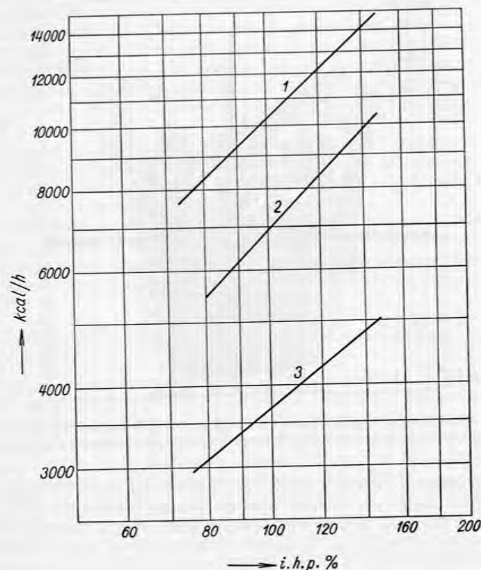
FIG. 52. Distribution of heat in the cylinder and head of an in-line Ranger aircraft engine in dependence on the indicated performance i.h.p. The temperature of the aluminium cylinder was maintained at 145 °C, cylinder head temperature varied between 216—275 °C. Air-fuel ratio and temperature of intake mixture was constant.
