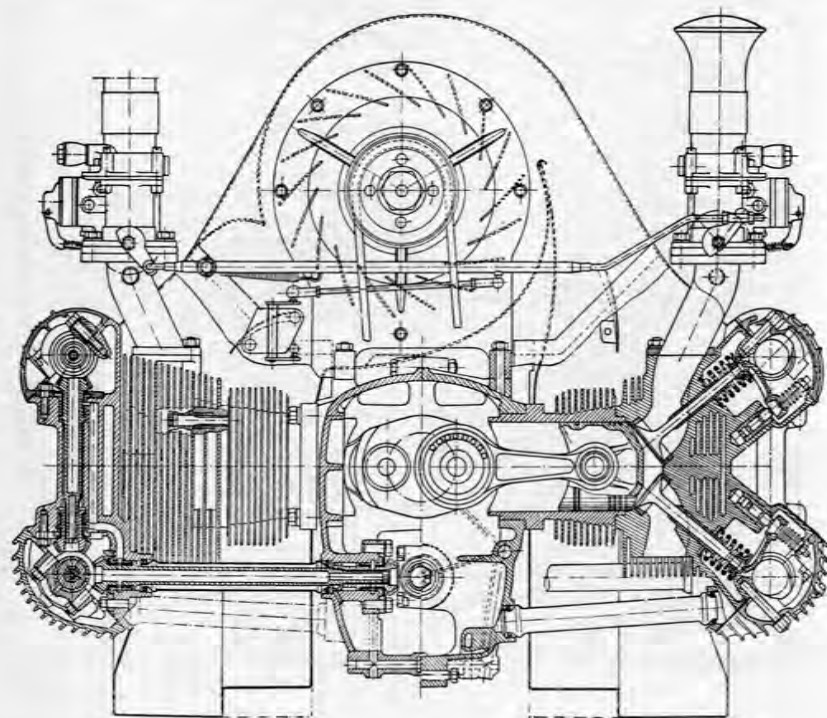
FIG. 380. Transverse section of the Porsche engine.
