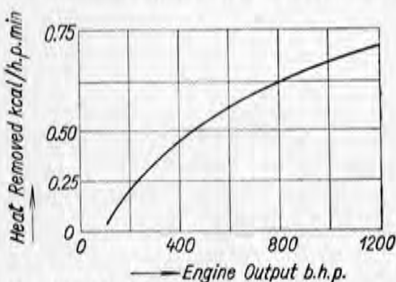
FIG. 329. Heat removed by oil in aircraft engines.
