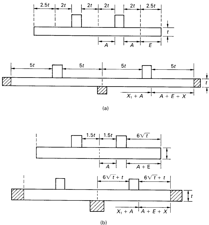
Figure 17.4 Feeding distance in steel castings: (a) Plate (width:thickness > 5:1 ) (b) Bar (width:thickness < 5:1 ).
