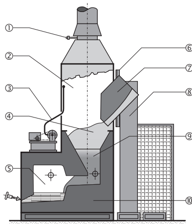
Figure 3.3 Gas-fired shaft furnace. The STRIKO ETAmox system. (Courtesy STRIKO UK Ltd.)
