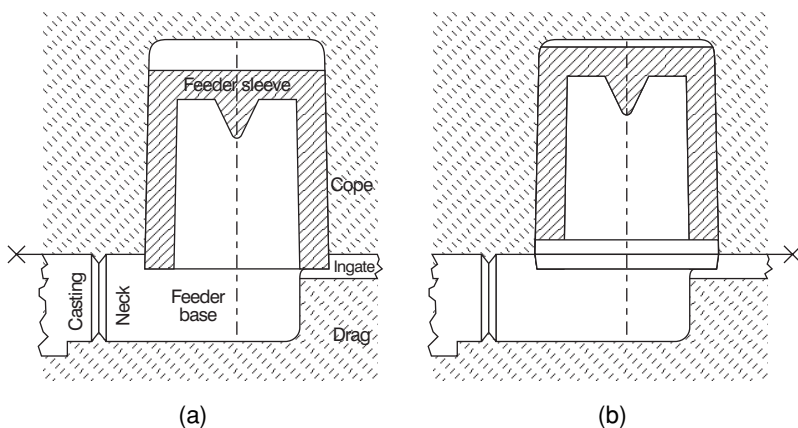
Figure 17.19 Floating sleeve functional principle.
