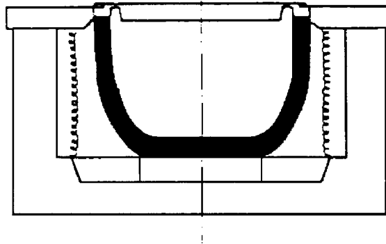
Figure 3.5 Electrically heated crucible furnace. (Courtesy Ramsell Furnaces Ltd, Droitwich.)
