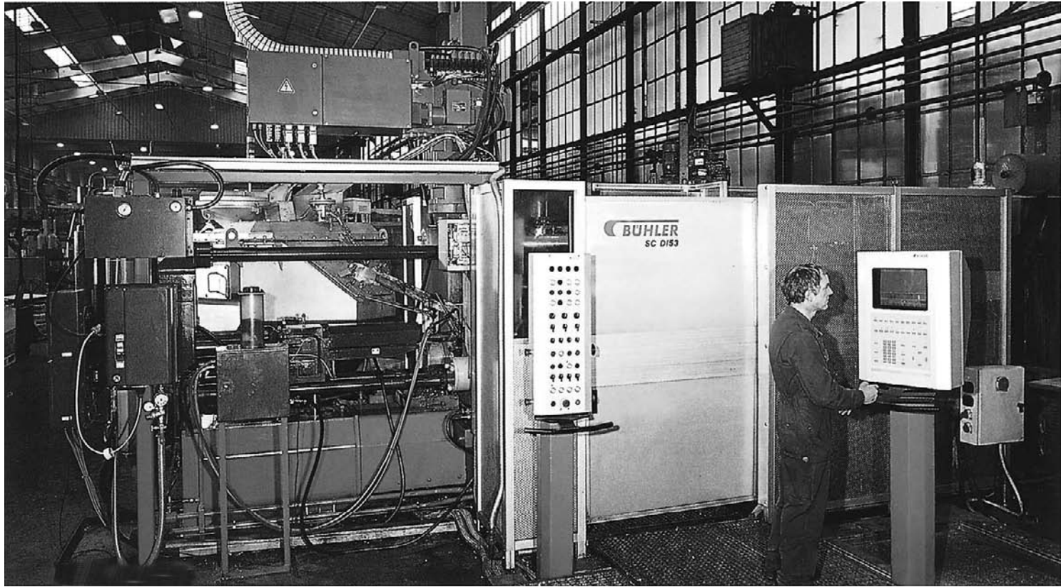
Figure 9.2 A Buhler SC D/53 pressure diecasting machine. Locking force 5250 kN, platen size 1080 \times 1080 mm with Real Time Shot Control SC. Suitable for Al castings of 2.3–6.5 kg shot weight. (Courtesy Buhler Ltd.)
