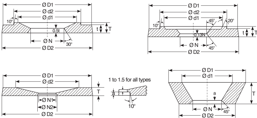
Figure 17.17 Standard forms of breaker cores.
