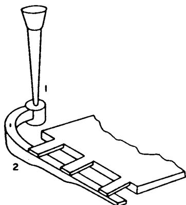
Figure 16.7 Gating high conductivity or commercial copper castings, multiple ingates. For castings of large surface area where more than one ingate helps to fill mould uniformly.
