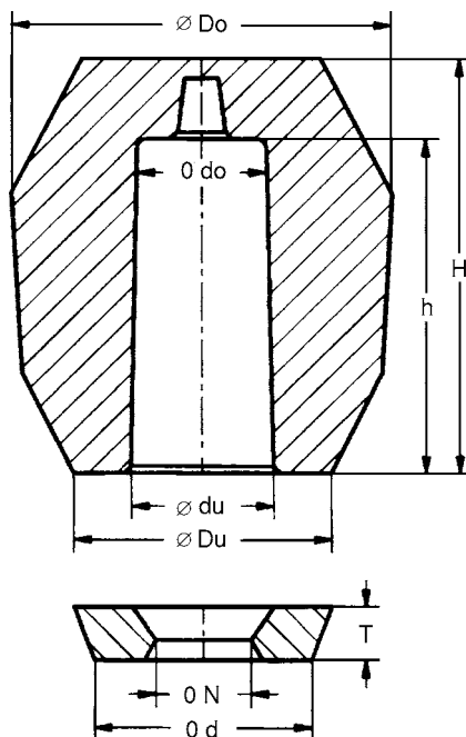
Figure 17.12 FEEDEX HD V-sleeve.
