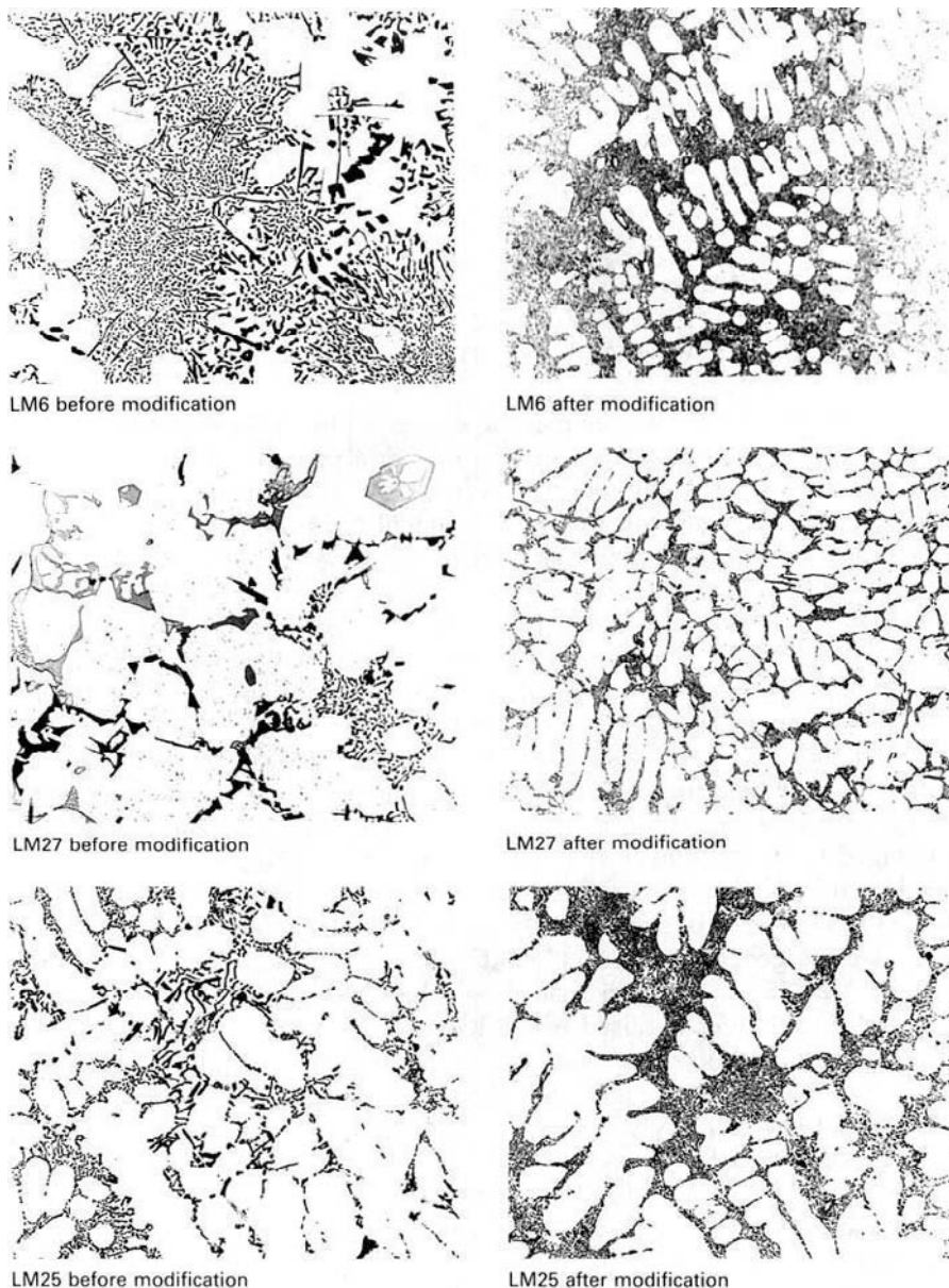
Figure 6.6 The effect of modification on the microstructures of aluminium alloys ( \times 125 ).
