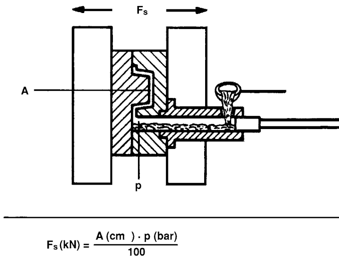
Figure 9.1 Calculation of the die opening force. (Courtesy Buhler Ltd.)
