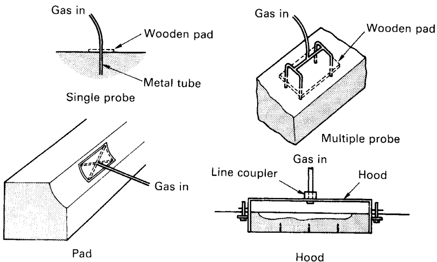
Figure 14.2 \text{CO}_2 -silicate process, methods of gas application.
