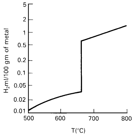
Figure 6.1 Solubility of hydrogen in aluminium.
