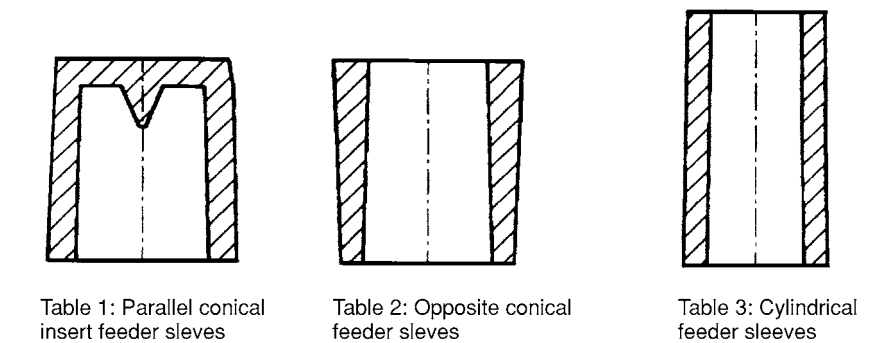
Figure 17.8 Foseco sleeve types.
