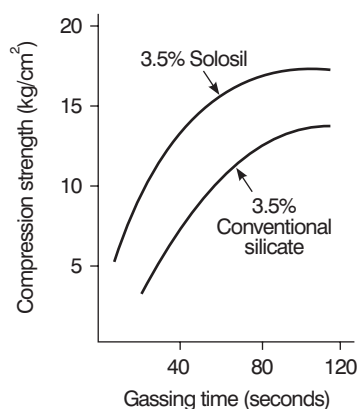
Figure 14.3 Strength development of SOLOSIL compared with conventional sugar/silicate system.
