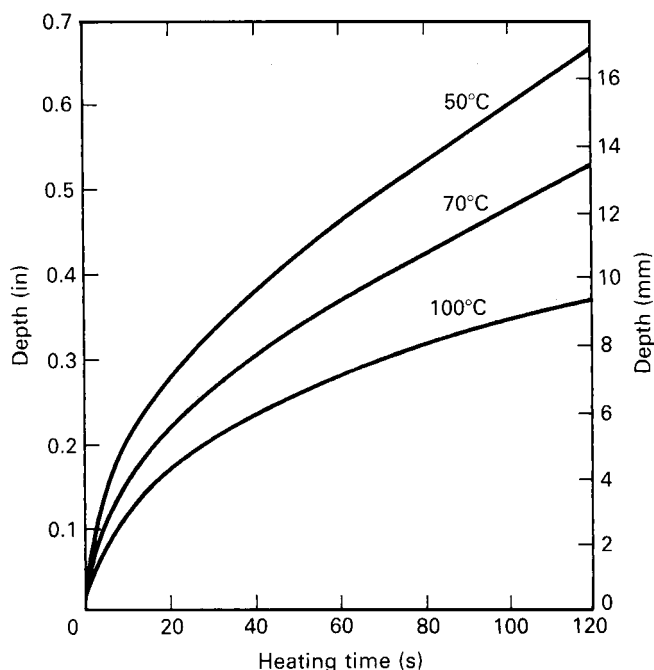
Figure 13.4 Temperature rise in a sand core with one surface in contact with a heated core box at 250°C (theoretical).
